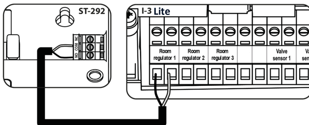
Example connection of a two-state regulator
