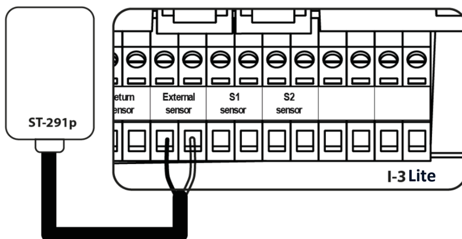
Connecting the external sensor
