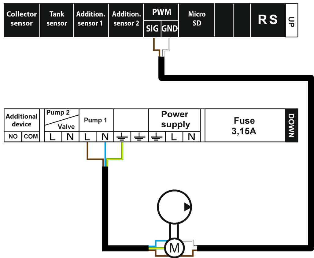
PWM pump connection scheme:
